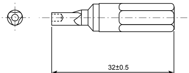
TR BIT FOR TRS [TRIO PIN USE]
