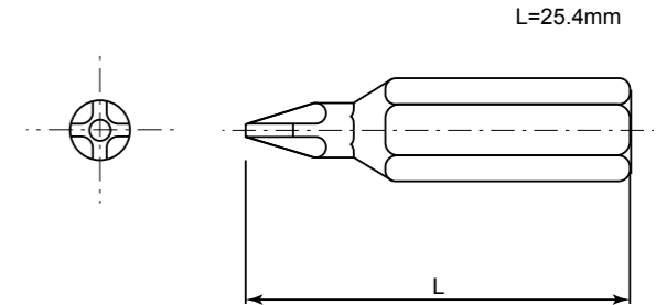
PP BIT FOR TRS [PHILIP PIN USE]
