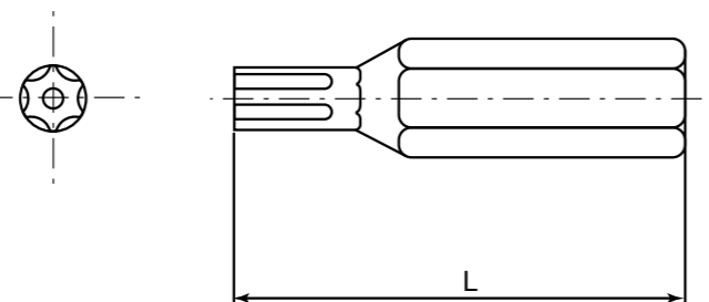
TP BIT FOR TRS [TORX PIN SHEET METAL USE - INCH]
