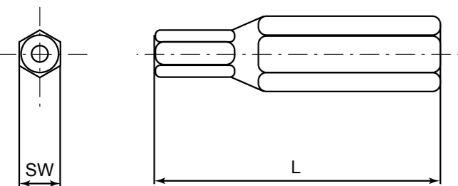
HP BIT FOR TRS [SOCKET PIN SHEET METAL USE - INCH]
