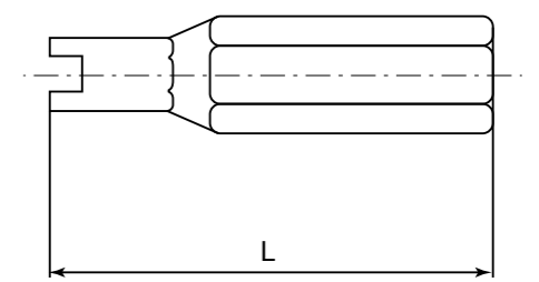
DS BIT FOR TRS [DRILL SPANNER SHEET METAL USE - INCH]
