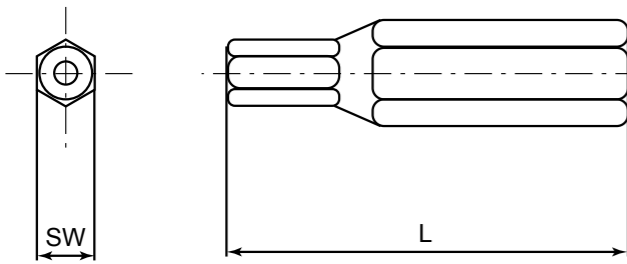
HP BIT FOR TRS [SOCKET PIN USE]
